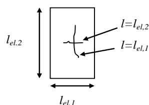
Figure I.3. Definition of the element length for different crack directions through an element.
