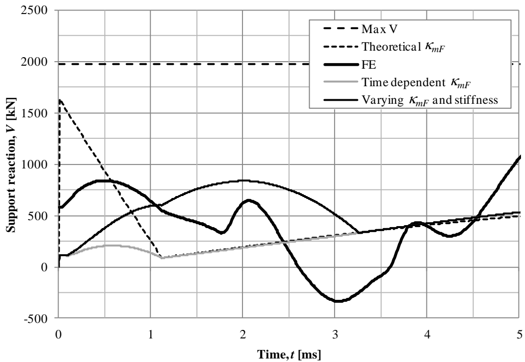
Figure 6.5. The early support reaction with the different methods for a load with peak pressure 5000 kPa and 1.12 ms duration.
