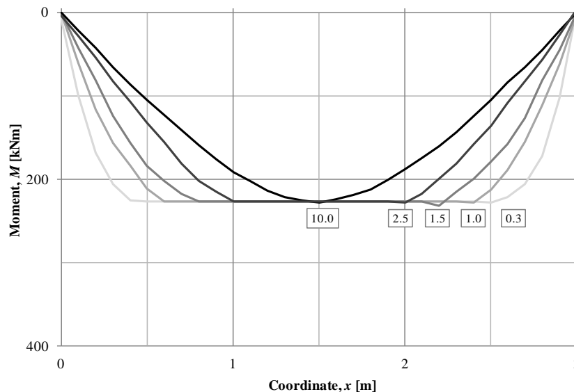
Figure 5.14. The moment distribution for different times in the ideal plastic case. The adjacent number denotes the time when the specific distribution occurs.
