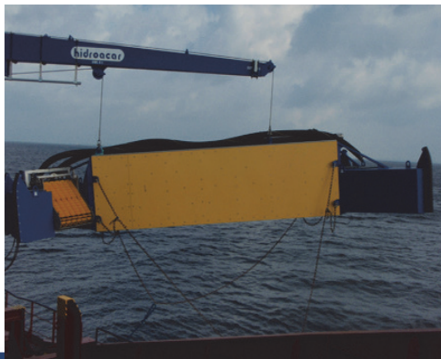
Sweeping arm
